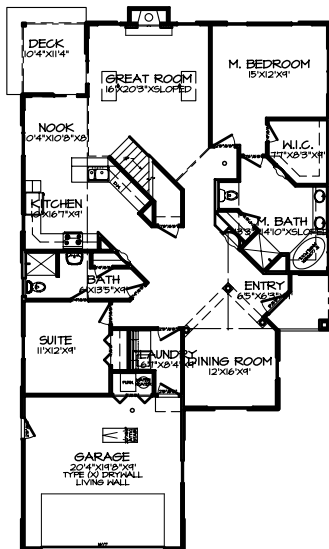
FIRST FLOOR PLAN SCALE: 1/8"=1'-0"
