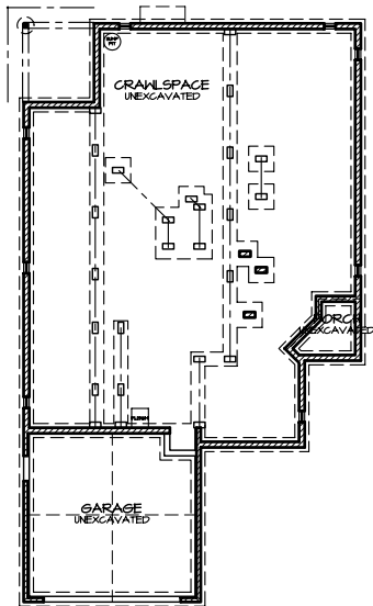
FOUNDATION PLAN SCALE: 1/8"=1'-0"
